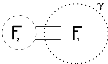
Figure 9. — The partition of \Pi induced by the splitting of \gamma .
