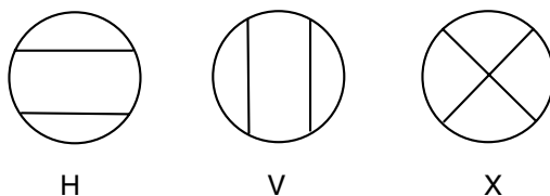
Figure 13. — Description of the connection paths H , V and X .
