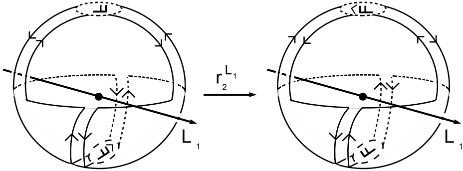
Figure 17. — The action of r_2^{L_1} .
