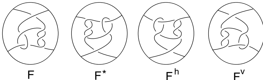
Figure 15. — A picture of the tangles F , F^* , F^h and F^v .
