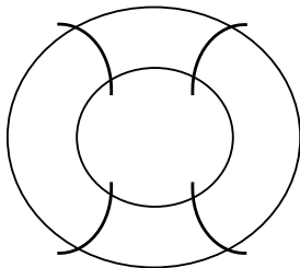
Figure 5. — Parallel Haseman circles.
