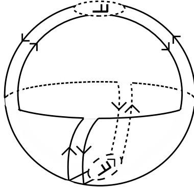
Figure 16. — A picture of \Pi on the 2-sphere.
