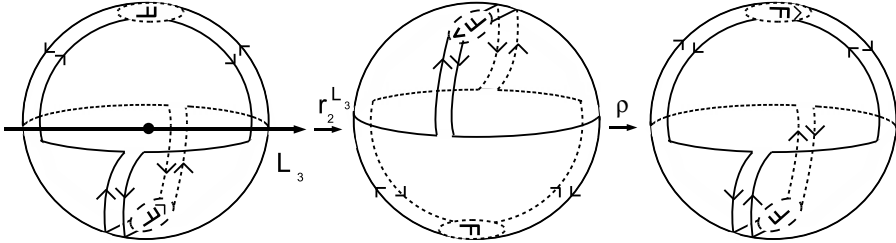
Figure 20. — The action of R_2^{L_3} .
