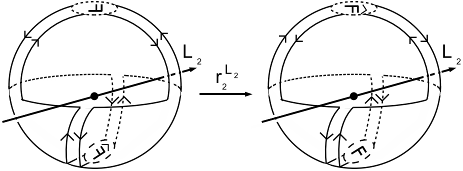
Figure 18. — The action of r_2^{L_2} .
