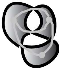
Figure 21. — A checkerboard graph.
