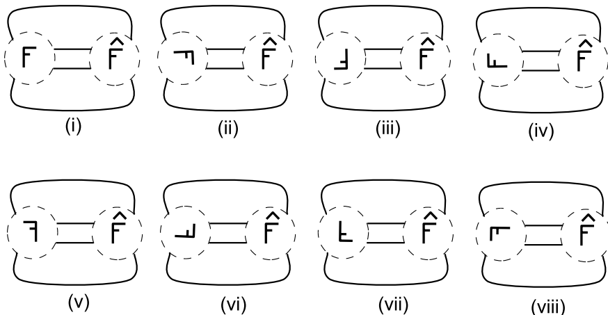
Figure 12. — The eight possible configurations.
