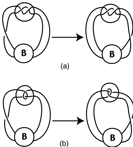
Figure 7. — (a) An inefficient flype (b) An efficient flype
