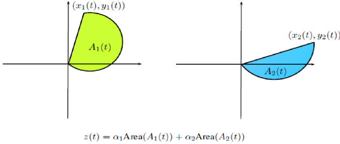
Figure 4.1. Projection of a non-horizontal geodesic: case 0 < \alpha_2 \leq \alpha_1
